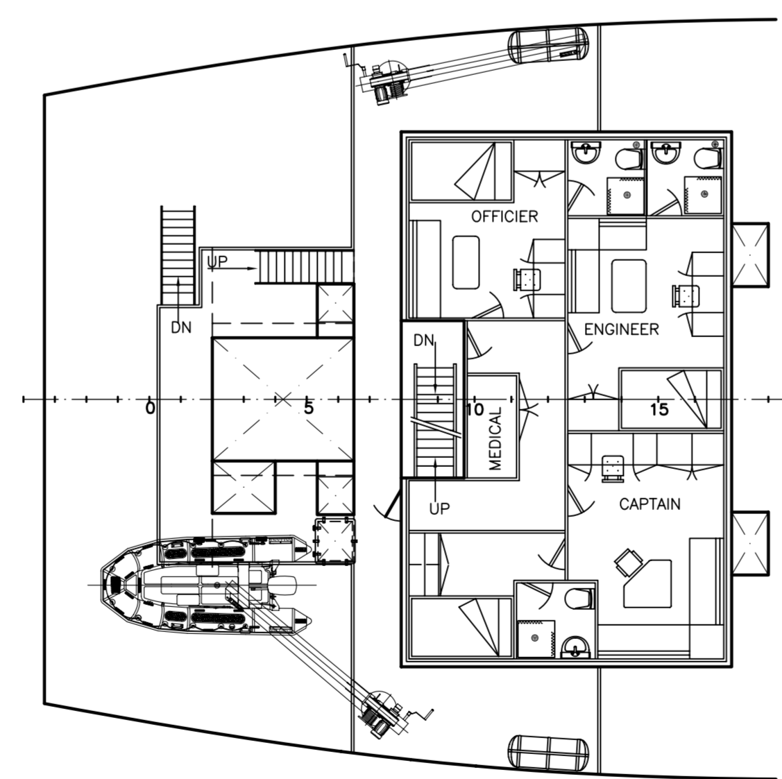
BOAT DECK
