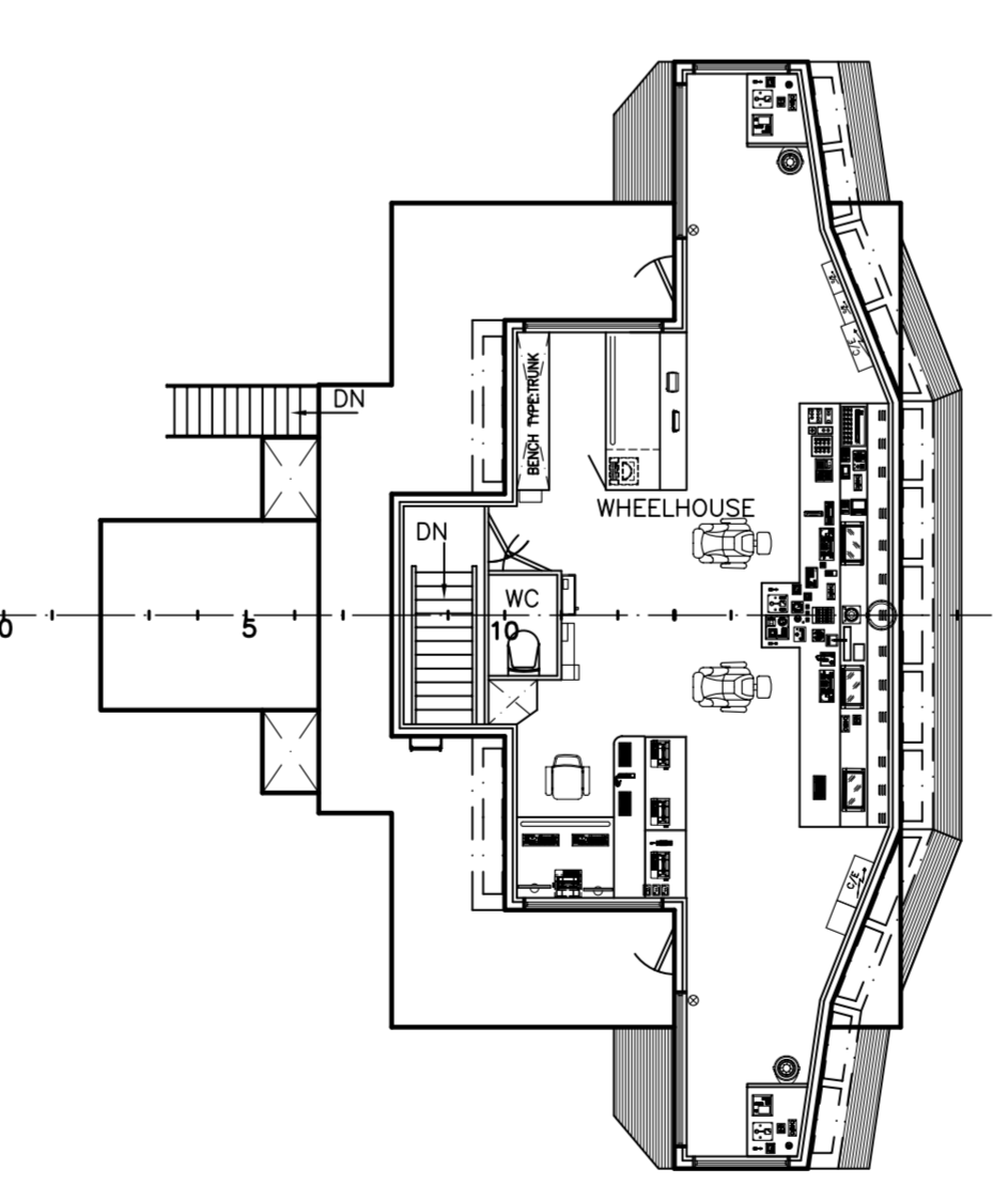
BRIDGE DECK
