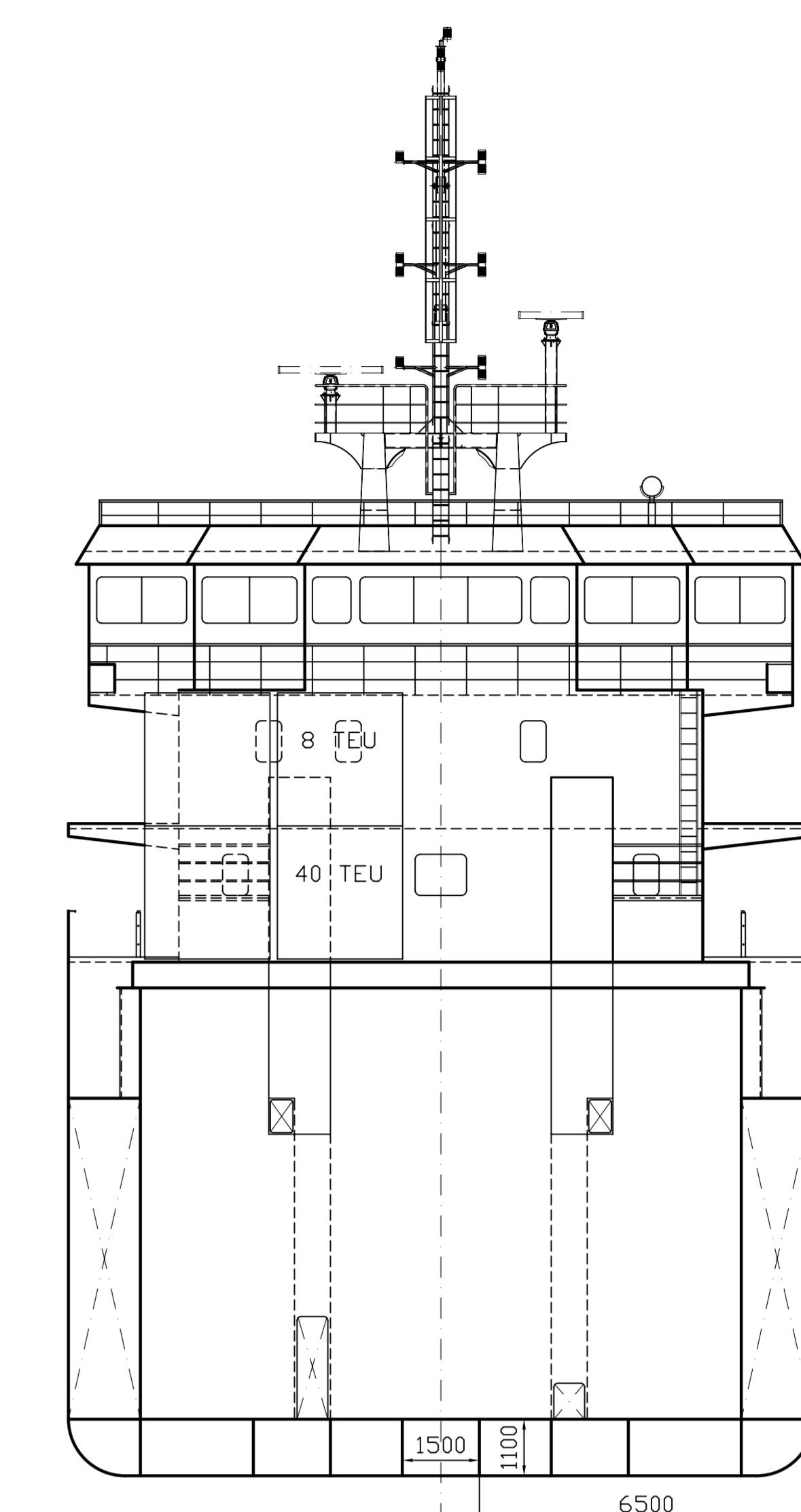
CROSS SECTION
