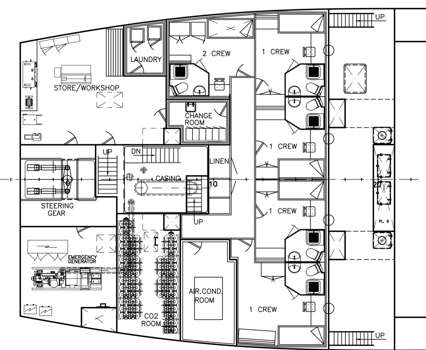
MAIN DECK
