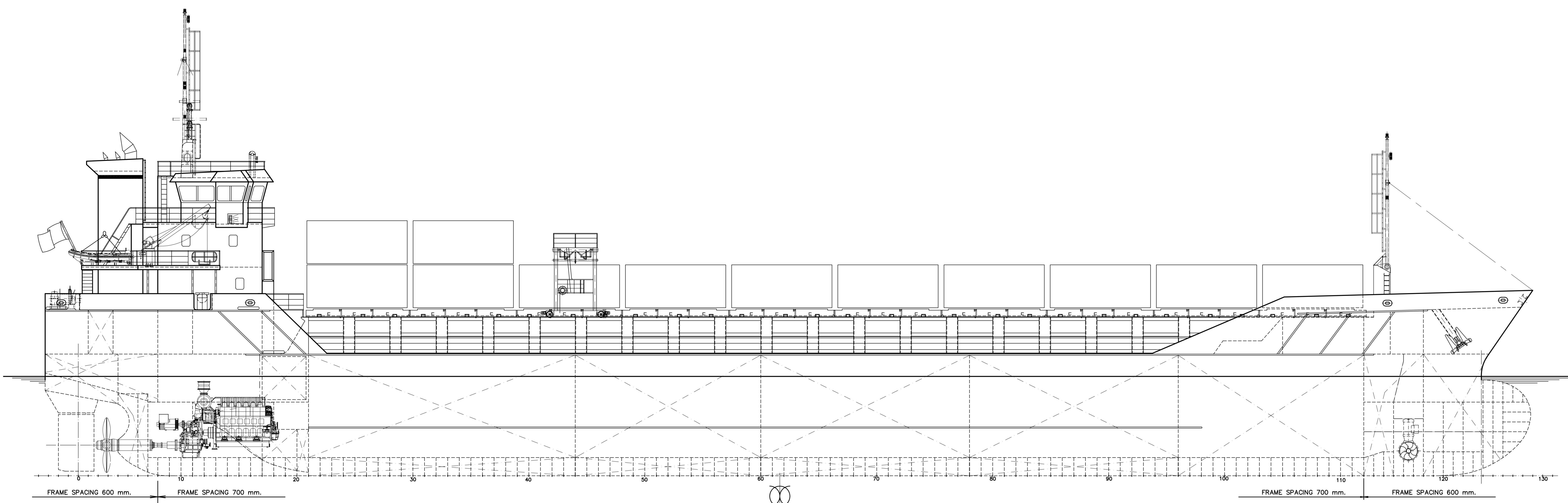
PROFILE
