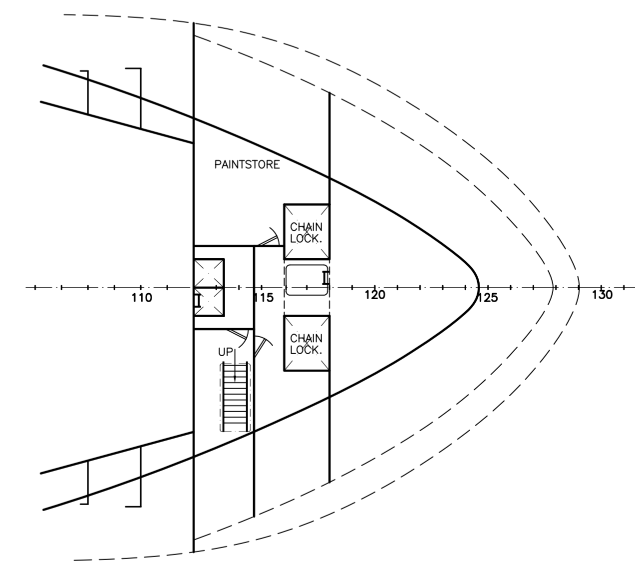
MAIN DECK
