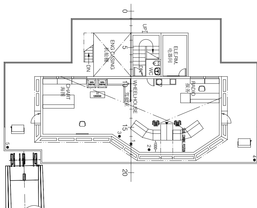
桥楼甲板 BRIDGE DECK 24850
